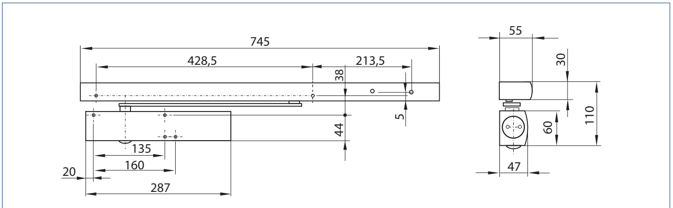
TS 5000 R
